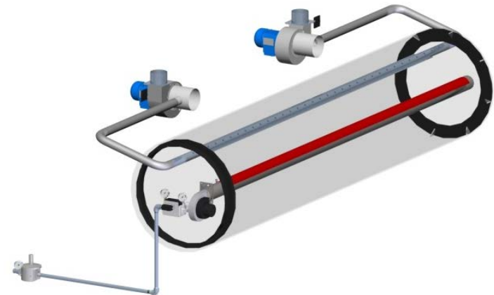
Radiant burners (New - Gas)
